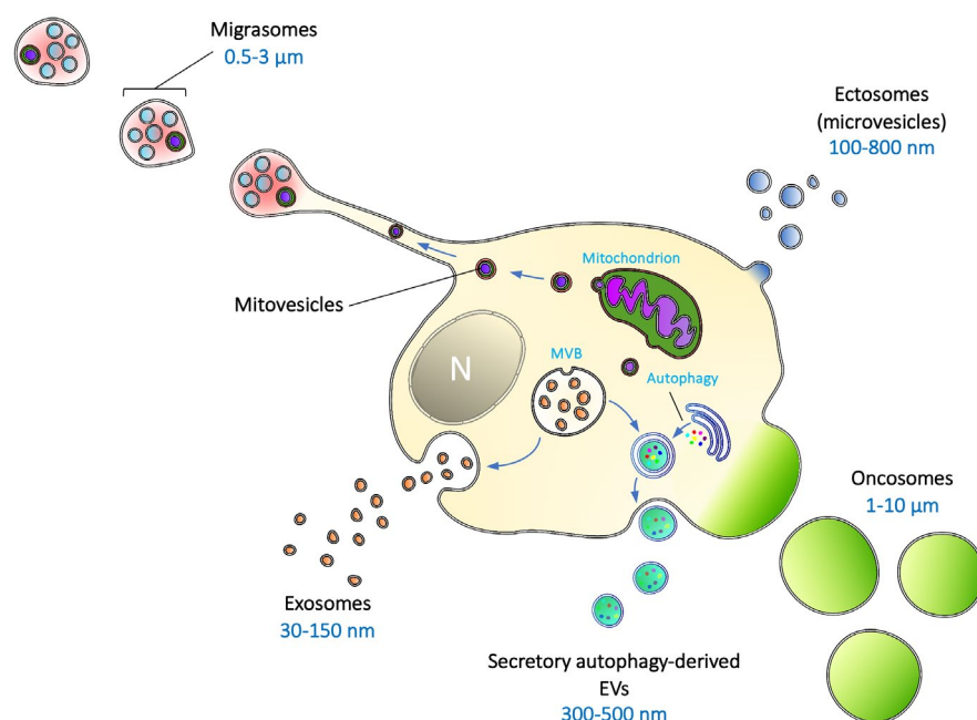
FIGURE 1 EV sub-populations released by a single cell, with their respective diameters. EV, extracellular vesicles; MVB, multivesicular body; N, nucleus
