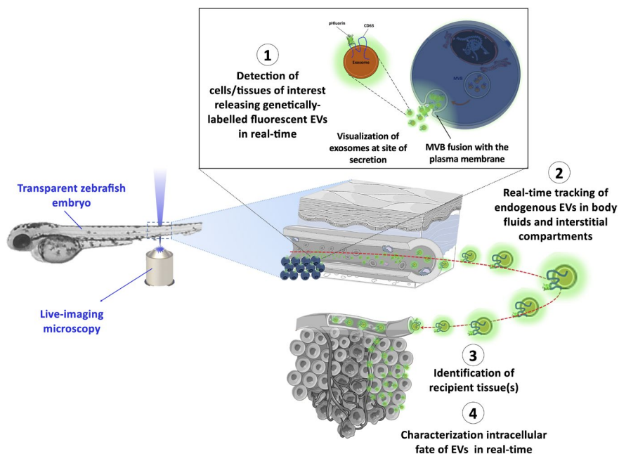
FIGURE 2 Zebrafish (ZF) embryos as comprehensive model to investigate EV-biology in vivo. Live-imaging of genetically labelled endogenous EVs in the ZF embryo allows to (1) study their release by producing cells, (2) follow their journey in the bloodstream and interstitial compartments, (3) follow their uptake by their natural targets and (4) characterize their intracellular fate. EV, extracellular vesicles
