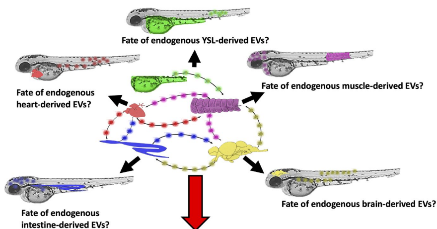
FIGURE 3 Visualization and mapping of the endogenous “inter organ EV-interactome” in the ZF embryo. Tissue-specific expression of EV (-subpopulation) reporter-proteins as well as cargo-transfer reporter systems could help unravel EV-mediated communication pathways existing between different tissues and organs. EV, extracellular vesicles; ZF, zebrafish
