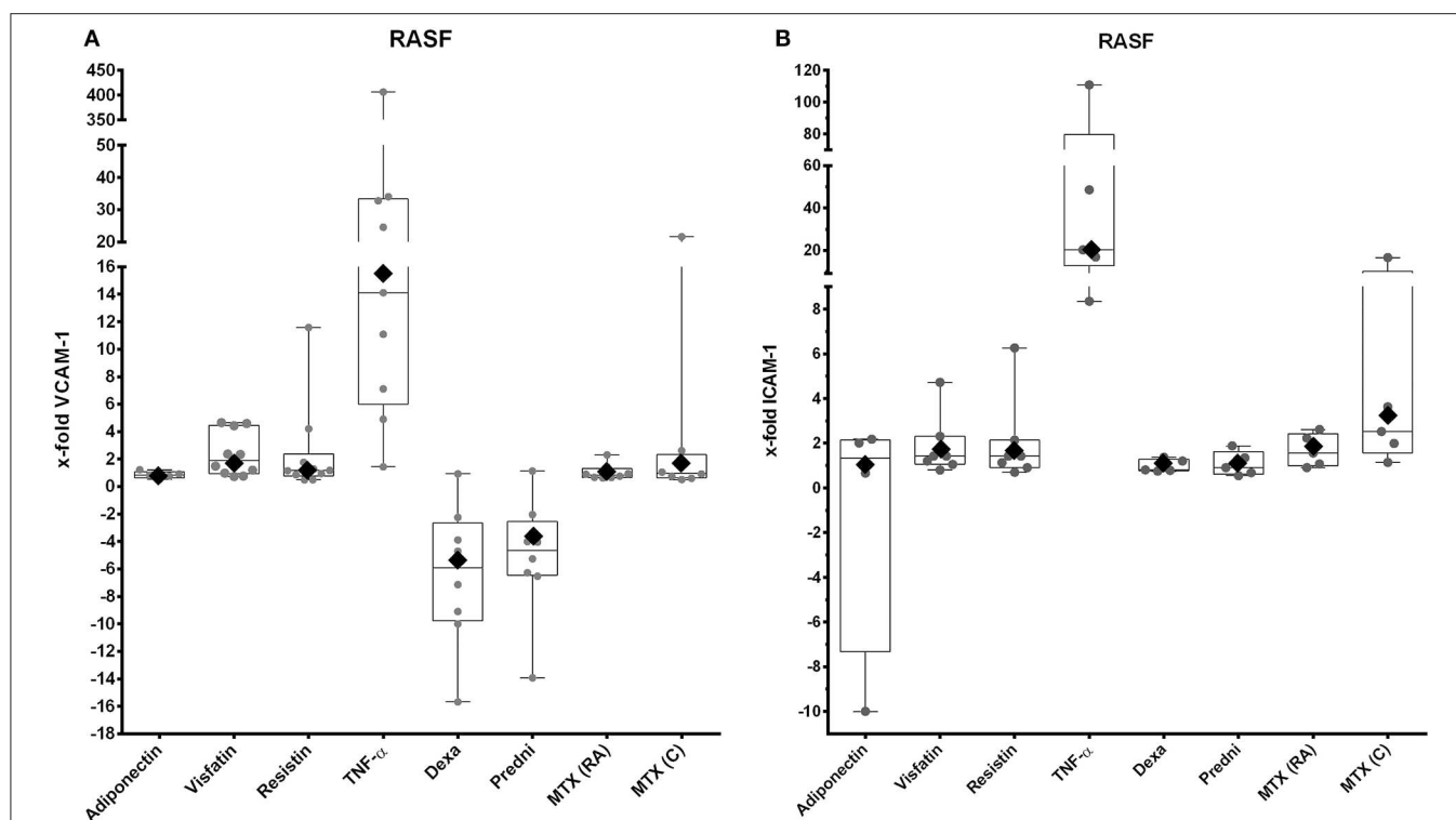
FIGURE 2 | VCAM-1 and ICAM-1 expression by RASFs after stimulation with selected adipokines and therapeutics. Results were compared to non-stimulated controls. (A) mRNA expression of VCAM-1 by RASFs after stimulation with adiponectin ( n = 5 ), visfatin ( n = 10 ), resistin ( n = 10 ), \text{TNF-}\alpha ( n = 9 ), or therapeutics ( n = 8 each). Adipokines and methotrexate did not have any effect on expression of VCAM-1, whereas \text{TNF-}\alpha upregulated expression of VCAM-1 [16.4-fold (rhombus), 95% CI = 4.9–55], but not significantly. Dexamethasone [–5.09-fold, 95% CI = 0.095–0.408] and prednisolone [–3.2-fold (rhombus), 95% CI = 0.14–0.717] downregulated expression of VCAM-1. (B) mRNA expression of ICAM-1 by RASFs after stimulation with adiponectin ( n = 4 ), visfatin ( n = 7 ), resistin ( n = 7 ), \text{TNF-}\alpha ( n = 5 ), and therapeutics (each n = 5 ). Adipokines and therapeutics did not have any effect on expression of ICAM-1. Tumor necrosis factor \alpha significantly upregulated expression of ICAM-1 [20.4-fold (rhombus), 95% CI = 6.07–68].
