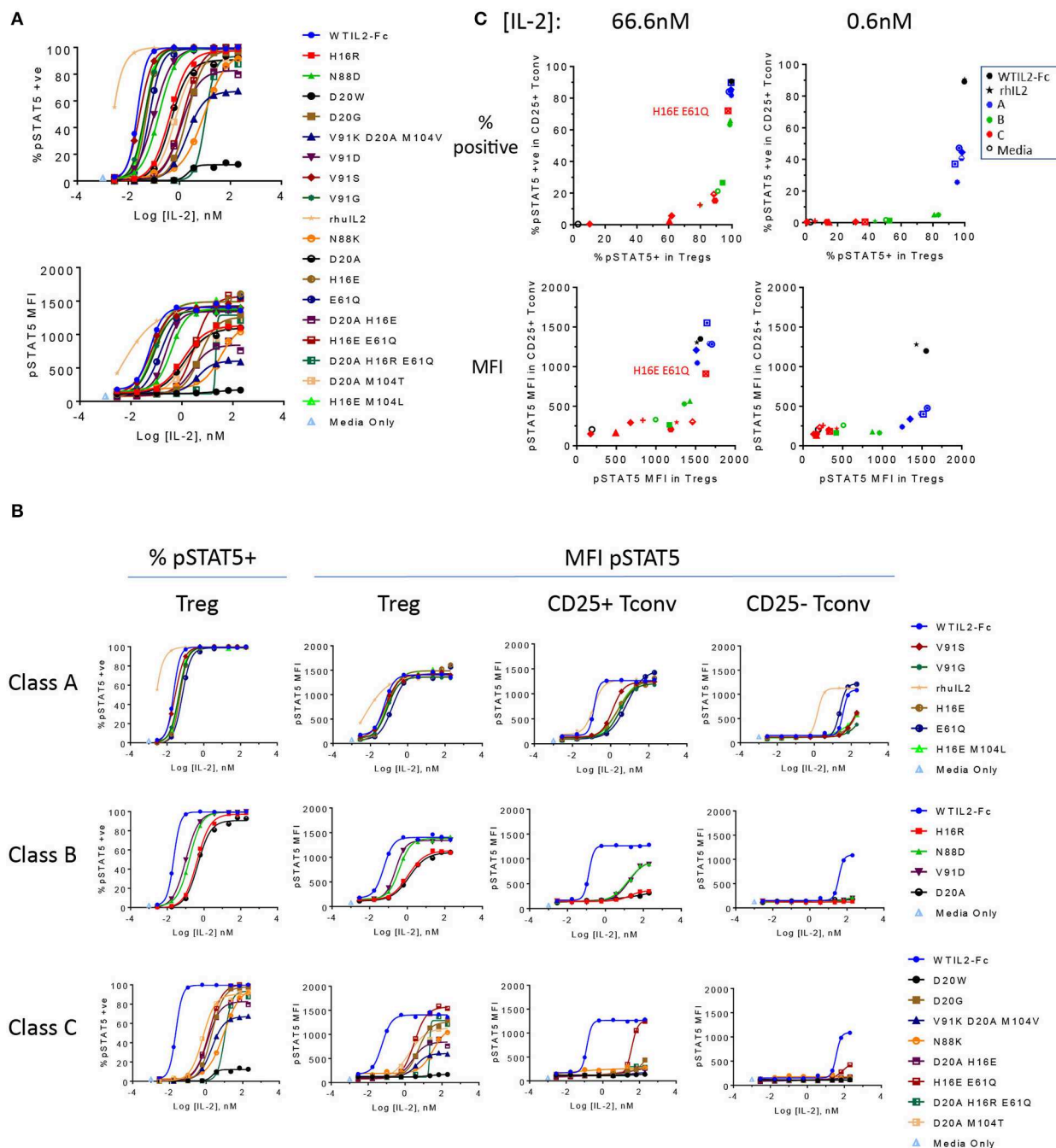
FIGURE 2 | The engineered IL-2 mutagenesis panel induces a broad spectrum of pSTAT5 response. (A) Activity of the individual IL-2 mutants is represented by phospho STAT5 (pSTAT5) signal at increasing concentrations of IL-2 mutants in human whole blood cell assay. pSTAT5 responses are shown as both the percent (%) pSTAT5-positive cells (top panel) and pSTAT5 MFI of (bottom panel) CD25hi Foxp3+ gated Treg cells (gating of an example plot shown in Supplementary Figure 1 ). Shown are representative plots of data from three donors. (B) The same pSTAT5 data shown in (A) are represented according to the potency-based classification to illustrate the impact of attenuation on various cell populations. Both the percent positive and pSTAT5 MFI for Treg gated populations are shown. In addition, pSTAT5 MFI data are shown for CD25+ Tconv, and CD25- Tconv cells. (C) The activity of the mutants on CD25+ Tconv cells vs. Treg cells are shown in 2D plots. Percent pSTAT5-positive and pSTAT5 MFI readouts at mutant concentrations 66.6 and 0.6 nM are shown, color coded to represent wildtype IL-2 as the Fc fusion (WTIL2-Fc, black circle), free recombinant cytokine (rhIL2, black star), class A (blue), B (green), C (red) mutants, and media only control (black open circle).
