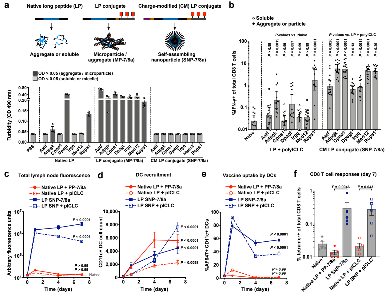
Fig. 4: SNP-7/8a improves formulation consistency, immunogenicity and PK compared to conventional PCV approaches. (a,b) Seven MC38 neoantigens known to bind MHC-I (Aatf, Adpgk, Cpne1, Dpagt, Irgq, Med12 and Repls1) were produced as either native LPs; conjugates of oligo-7/8a that form microparticles/aggregates (MP-7/8a); or charge-modified (CM) conjugates of oligo-7/8a that self-assemble to nanoparticles (SNP-7/8a). (a) Turbidity of the LP formulations ( n = 3 per composition) at 0.5 mg/mL in PBS pH 7.4 was assessed by measuring absorbance (optical density (OD), arbitrary units) at 490 nm; turbidity > 0.05 indicates aggregation. (b) C57BL/6 mice ( n = 12-15 per group) were injected subcutaneously with native LPs admixed with polyICLC and anti-CD40 or SNP-7/8a on days 0 and 14, and CD8 T cell responses were assessed from blood by intracellular cytokine staining on day 28. (c-f) C57BL/6 mice ( n = 5 per group per time point) were injected subcutaneously with fluorophore (AF647)-labeled Cpne1 neoantigen as either a native LP admixed with a particle adjuvant (polyICLC or PP-7/8a) or as a self-assembling nanoparticle (SNP) admixed with polyICLC or co-delivering TLR-7/8a (SNP-7/8a). Lymph nodes ( n = 10 per group per time point) draining the site of immunization were collected at serial time points and assessed for (c) total tissue fluorescence (peptide quantity), (d) total CD11c+ DC count and (e) the percentage of total CD11+ DCs that had taken up vaccine (AF647+). (f) CD8 T cell responses from blood were assessed by tetramer staining on day 7. Data on log scale are reported as geometric mean with 95% c.i.; data on linear scale and all line graphs are reported as mean \pm s.e.m. Statistical significance was determined using Kruskal-Wallis with Dunn's correction (b,f) or two-way ANOVA with Bonferroni correction (c-e).
