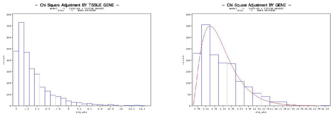
(c) Distribution chi2 of variances
