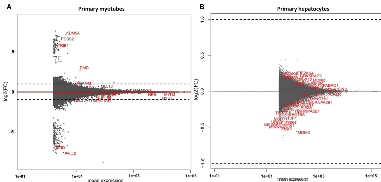
Figure 6. Exon Junction Usage Analyzed Using DEXseq
