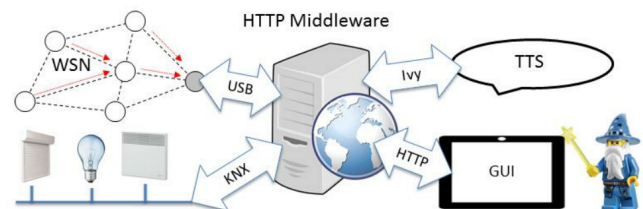
Figure 1: MIOZ platform.
