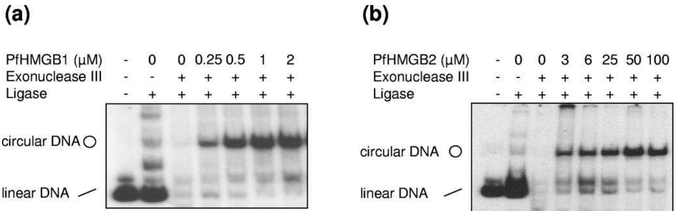
FIG. 3. DNA bending and ligase-mediated circularization assay with either rePfHMGB1 (a) or rePfHMGB2 (b). The \gamma\text{-}^{32}\text{P} 5' end-labeled 123-bp DNA fragment was preincubated with increasing amounts of rePfHMGB1 (0 to 2 \mu\text{M} ) or rePfHMGB2 (0 to 100 \mu\text{M} ), followed by ligation with T4 DNA ligase. The ligation products were subjected to electrophoresis after exonuclease III treatment. T4 DNA ligase was added to all samples except that loaded in the first lane. All samples were treated with exonuclease III except samples of the first two lanes. The migration positions of 123-bp linear and 123-bp minicircular DNAs are indicated at left.
