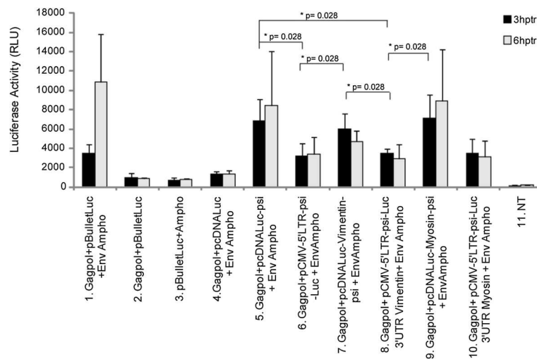
Figure 6 Luciferase activity upon retroviral transfer of mRNA into 293FT cells. 293FT cells were transduced with 100 \mu l supernatants containing retroviral particles harvested 48 h post-transfection. 3 or 6 h post-transduction, cells were lysed and luciferase activity was measured. We observed a statistically significant difference between the control condition 4 and all the test constructs (5 to 10) (p-value < 0,03). Statistical comparisons between the different constructs were performed on the 3 hours time-point and evaluated using a Wilcoxon-Mann-Whitney analysis. hptr, hours post-transfection. NT: untransfected cells. Number of experiments, N = 3.
