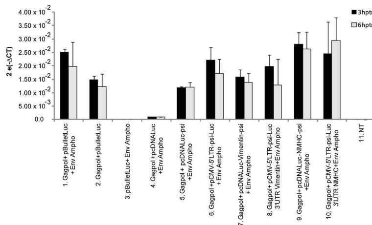
Figure 5 Retroviral transfer of mRNA into 293FT cells using relative RT-qPCR analysis. Quantitative RT-PCR analysis of luciferase mRNA levels in 293FT cells, 3 and 6 h post-transduction with retroviral particles harvested 48 h post-transfection, in each condition the luciferase mRNA was normalized to that of β-actin. Comparisons were performed using Wilcoxon-Mann-Whitney analysis, despite a tendency, no statistically significant differences could be observed. NT: untransfected cells. Number of experiments, N = 3.
