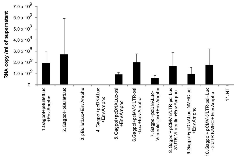
Figure 4 Recruitment of the modified mRNA into retroviral particles. Quantitative RT-PCR analysis of luciferase-mRNA content extracted from retroviral particles produced in cells transfected with the packaging constructs and the test-constructs, 48 h post-transfection. All results were normalized for transfection-efficiency with GFP expression determined by FACS analysis. Comparisons were performed using Wilcoxon-Mann-Whitney analysis. NT: untransfected cells. Number of experiments, N = 3.
