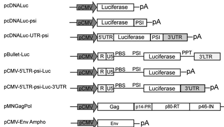
Figure 1 Schematic representation of luciferase vectors used for recruitment into retroviral particles. psi: MLV packaging signal. PBS: retroviral primer binding site. PPT: polypurine tract, priming + strand synthesis following the first jump during reverse transcription. pA: Bovine Growth Hormone polyadenylation signal. The last two constructs (pMNGag-Pol and pCMV-Env-Ampho) were used for transcomplementation in order to drive particles formations.
