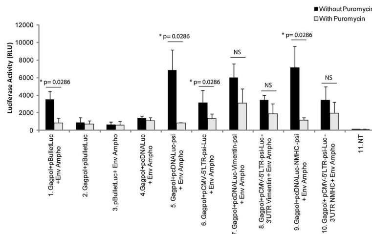
Figure 7 Luciferase activity upon retroviral transfer of mRNA into 293FT cells with and without translation inhibitor. 293FT cells were transduced with 100 \mu l supernatants containing retroviral-particles with or without 3 \mu g/ml puromycin. After 3 h, cells were lysed and luciferase activity was measured. Results were normalized by transfection efficiency with GFP expression by FACS analysis. The significance of the differences observed between the two conditions was determined by a Wilcoxon-Mann-Whitney analysis. NS : Not Significant. NT: untransfected cells. Number of experiments, N = 3.
