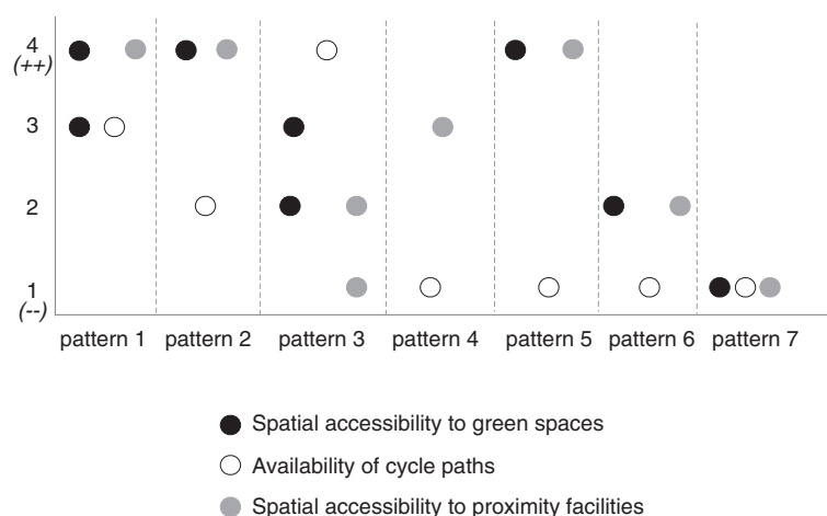
Figure 2 Characteristics of the seven built environmental patterns according to categories of spatial accessibility to green spaces, proximity facilities and availability of cycle paths. On the y axis are represented the 4 categories used for each variable. For green spaces and proximity facilities, the top and bottom quartiles represented high (++) and low accessibility (--). For cycle paths, (--) represented neighborhoods without cycle paths and the three other categories were defined using tertiles. Dots indicate those categories overrepresented in each cluster compared to the overall sample. For example, for Pattern 1, both quartiles 3 and 4 for spatial accessibility to green spaces were overrepresented.
