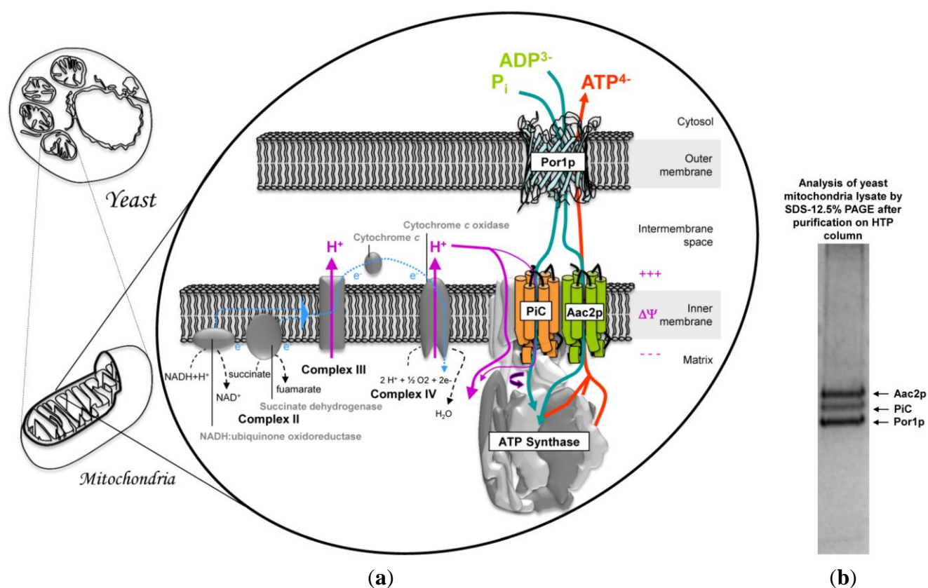
Figure 4. Machinery model of active transport driven by the electrochemical gradient of protons across the mitochondrial membranes. (a) The inorganic phosphate ( P_i ) and ADP^{3-} are imported into the matrix via two carriers: Aac2p and PiC while the matrix ATP^{4-} is consumed by the ATP synthase, shown in its monomeric form. The charge of each transported molecule is indicated. The membrane potential is negative in the matrix. The outer membrane ensures free passage of these compounds through the VDAC, noted Por1p; (b) Gel electrophoresis showing the co-purification of Aac2p, PiC and Por1p from a yeast mitochondria lysate in n-dodecyl- \beta -D-maltoside/emulphogen mix (DDM/EM) after chromatography on a hydroxylapatite column (Coomassie Blue staining of the SDS-PAGE gel).
