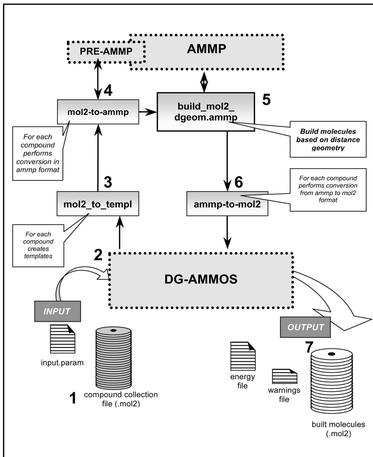
Figure 1 Schematic diagram of the DG-AMMOS algorithm. The arrows show the cycle for the automated procedure explained in details in the Implementation section.
