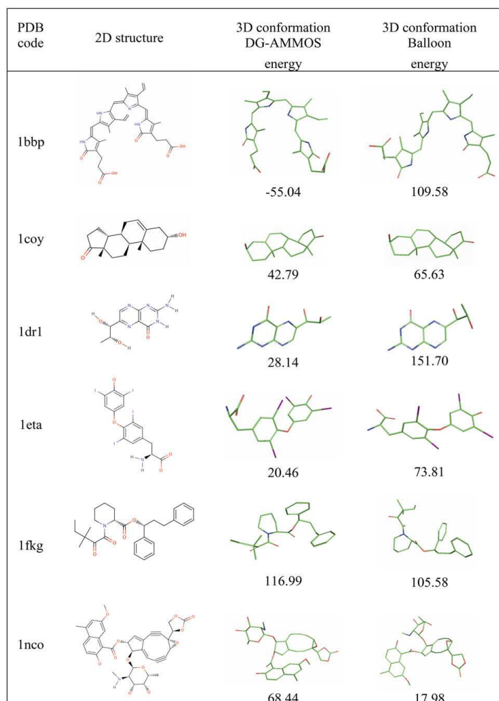
Figure 3 Examples of several compounds of the selected 114 molecules from the Astex Dataset with generated 3D conformations by DG-AMMOS and Balloon. The energies of the generated single 3D conformations (not necessarily the lowest energy ones) are shown in kcal.mol -1 .
