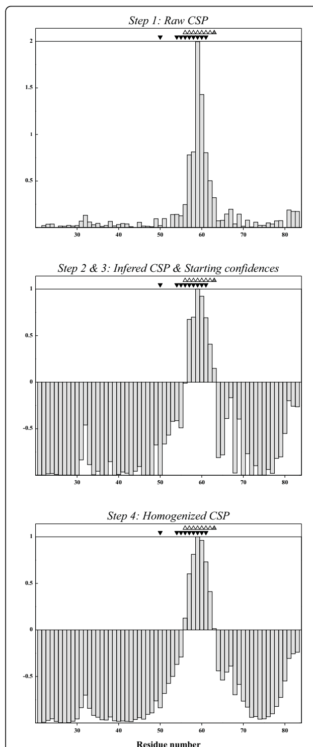
Figure 1 Chemical shift perturbations and derived confidences as function of the residue sequence for CI2 (unbound and bound to BPN'). Top: Raw CSP data; Middle: Starting confidences; Bottom: Confidences after homogenization. The triangles filled in black show residues involved in the interaction between CI-2 and BPN', the ones filled in grey show the selection made by SAMPLEX and the open ones, residues in an intermediate state.
