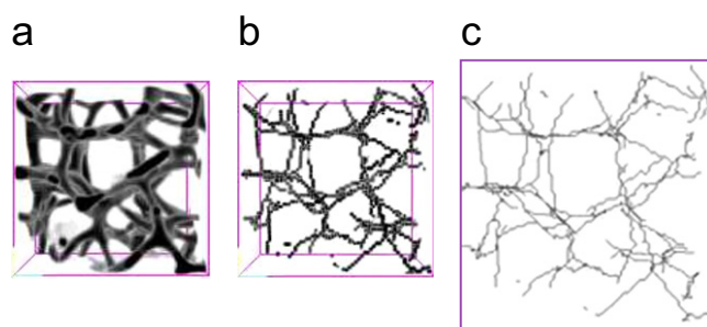
Fig. 6. Example of skeleton. (a) Initial tomography volume, (b) skeleton based on wall reducing (homotopic thinning technique) and (c) corresponding finite element, using beam element.
