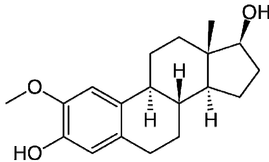
2-methoxyestradiol
