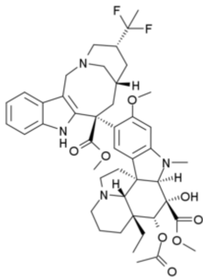
Vinflunine
