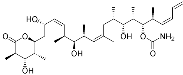
Discodermolide
