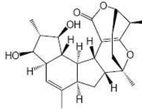
Cyclostreptin
