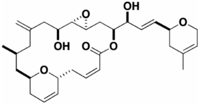
Lulimalide
