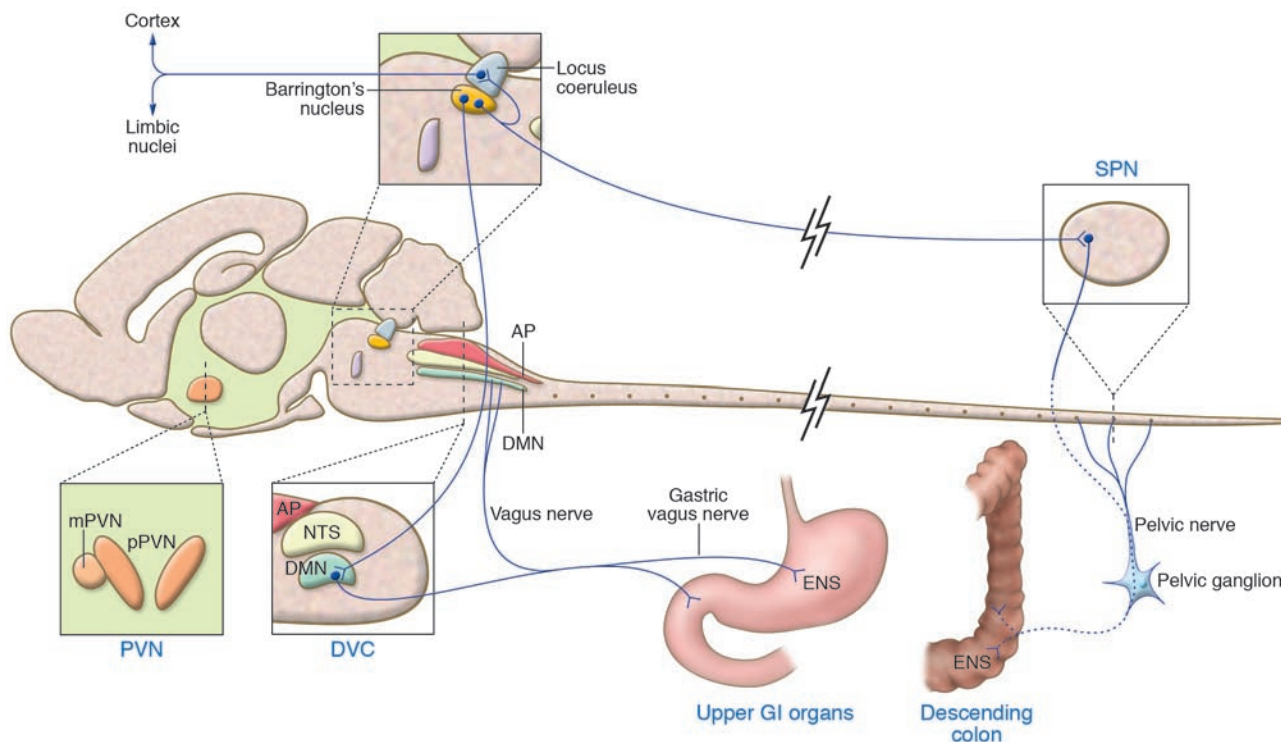
Figure 2 Lengthwise drawing of the rat brain showing the regions in which the activation of receptors for CRF influences gastric and colonic motor function through neural pathways innervating the gut. The Barrington's nucleus, through its reciprocal connections with the LC, can be influenced by or influence the noradrenergic-containing neurons in the LC that project to the forebrain. Efferent fibers from the Barrington's complex also project to neurons in the dorsal motor nucleus (DMN) and the sacral parasympathetic nucleus (SPN). Axons from DMN neurons provide vagal innervation to the stomach. The end target of vagal efferent fibers is the enteric nervous system (ENS) in the stomach wall. Stress activates the PVN, LC, and Barrington's nucleus, resulting in autonomic nervous system-mediated inhibition of gastric and stimulation of colonic transit and motility. Vertical lines indicate coronal sections at the PVN and dorsal vagal complex (DVC). AP, area postrema; GI, gastrointestinal; mPVN, magnocellular PVN; NTS, nucleus tractus solitarius; pPVN, parvocellular PVN. Adapted with permission from Trends in Pharmacological Sciences (ref. 91; Figure 1).
