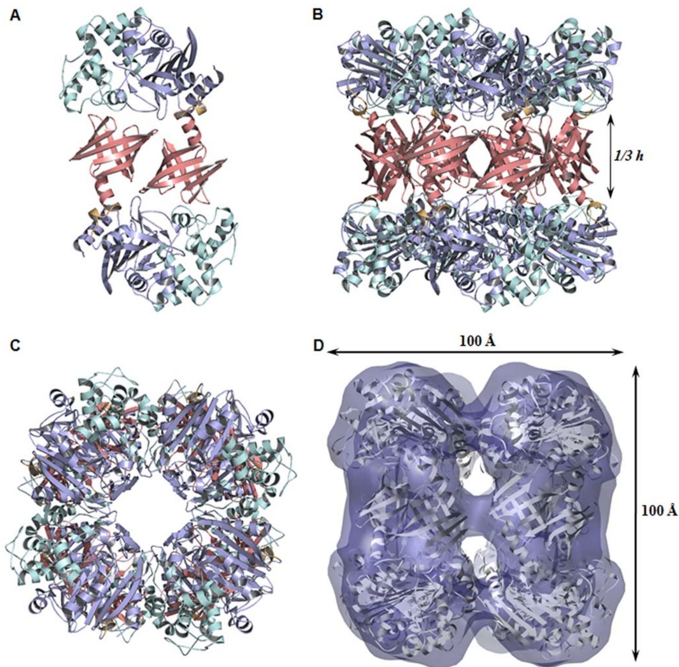
Figure 2. The CubicO particle. Structural regions are color coded as in Figure 1. A , Ribbon representation of the head-to-tail dimer structure forming the edges of the cubic-shaped octamer. B , side view along and C , top view perpendicular to the four-fold axis of the octamer. The central ring formed by the C-terminal domains represents one third of the total height. D , Fitting of cryo-EM map shown in transparent solid surface with the X-ray structure.
