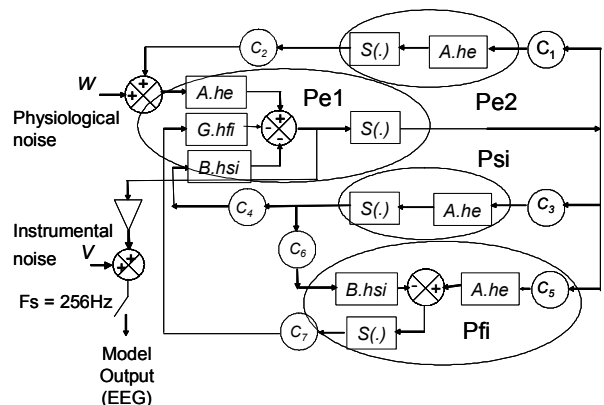
Fig. 1. The SEEG model.
