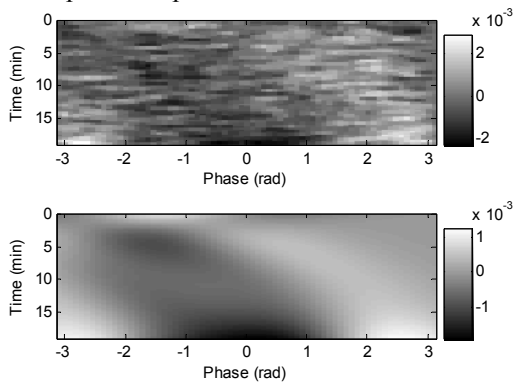
Figure 5: Two-dimensional SMS (top) and its fitted surface by F_3(t, \varphi) (bottom) in gray-level. SMS graphs are related to a patient during the 20 minutes of EEG recordings before surgical operation.
