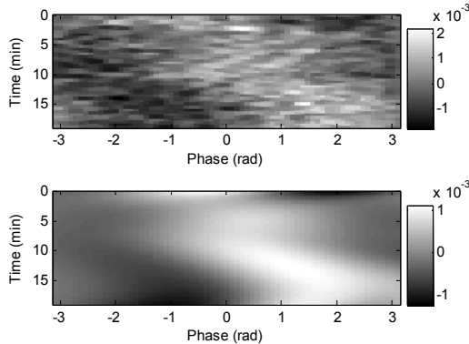
Figure 6: Two-dimensional FMS (top) and its fitted surface by F_3(t, \varphi) (bottom) in gray-level. FMS graphs are related to the same patient described in figure 5.
