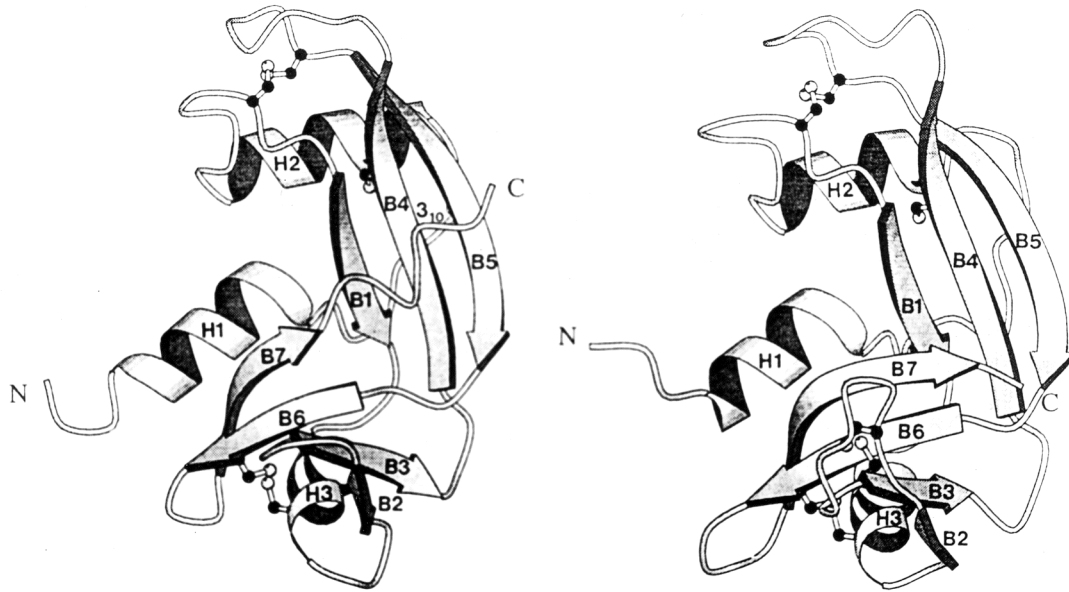
Figure 1. Three-dimensional structure of human angiogenin (Left) and RNase A (Right). MOLSCRIPT diagram reproduced with permission from [44] (Copyright 1994, Proc. Natl. Acad. Sci. USA).
