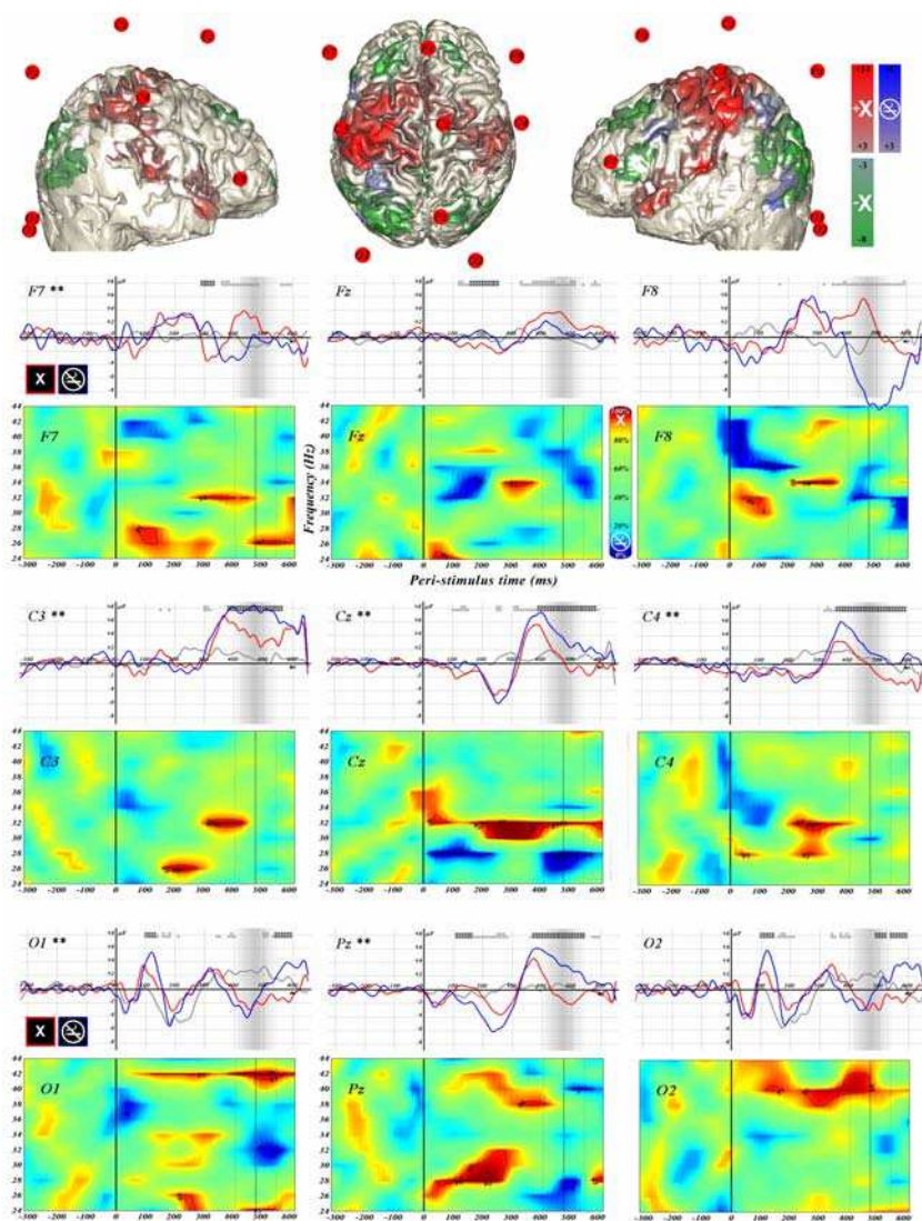
Figure 2 Evoked potentials and event-related oscillations for each electrode and for all the subjects. The upper part presents three different views of the average electrode position relative to the areas with BOLD activation (threshold p \leq 0.001 , 100 voxels, Target-related activation – red, Target-related deactivation – green, and rare Distractor (Novel) activation – blue). It is provided for better appreciation of electrical signals, considering fMRI activation. The lower part displays the evoked potentials (EPs) and event-related oscillations (EROs) for each electrode, for the 5 subjects. For C3, Cz, C4, Pz, the "no-smoking" symbol, which is an instance of Novels (blue), yielded larger EPs than Targets (red). Distractors are represented in gray. For all the electrodes, the reverse is true as far as EROs are concerned, with significantly more oscillations around 300–400 ms, regarding Targets. In the case of EPs, signals have been plotted from -325 to +625 ms and the voltage range was kept constant from -9 to +9 \mu\text{V} . The shaded region around 474 ms corresponds to the response time and its standard deviation. The statistics for the comparison of Target-related and Novel-related EPs are computed every 10 ms, between 100 ms and 600 ms, and represented by the gray and black stars above the curves (1 star for p_{nc} \leq 0.05 , 2 stars for p_{nc} \leq 0.01 ). The time-cluster significance, corrected for multiple comparison is indicated by the color of the stars: black if above p_c \leq 0.05 , gray if not significant at the corrected time-cluster level. The set level is given for each electrode by the number of stars beside the electrode label (1 star for p \leq 0.05 , 2 stars for p \leq 0.01 ). For EROs, only the statistics comparing Targets and Novels is given for the 24- to 44-Hz band, and between -320 to 600 ms. The solid and dotted black lines correspond to the response time and standard deviation, respectively. The color code for the statistics is shown on the upper right hand side, and represents the cumulative p distribution stated in percent. Cold colors code for a higher Novel-related power level, and hot colors code for greater Target-related power intensity. Regions above the .05 and .01 thresholds are contoured in black (notice that the numbers 1, 5, 95 and 99 represent the cumulative p values stated in percent).
