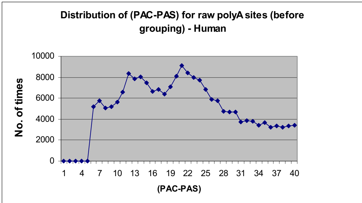
Figure 3 Distribution of spacing between polyA cleavage (PAC) site and polyA signal (PAS) in human transcript patterns from AltTrans. The bottom inset uses the data set of heterogeneous polyA sites; the top inset uses the data set of representative polyA sites (Nearby heterogeneous polyA sites are grouped and a representative polyA site is chosen – see text for methods).
