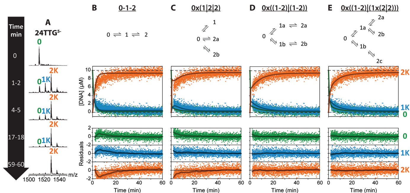
Figure 4. Kinetics of K + -binding (20°C) monitored by mass spectrometry of 10 μM 24TTG in 100 mM TMAA after adding KCl to reach a final concentration of 500 μM. (A) Mass spectra after addition of KCl at different time (integrated over 1 min accumulation). (B–E) Concentration of the complexes with 0, 1 or 2 potassium in green, blue and orange, respectively, as a function of time after K + addition. The data were fitted using the models described above each graph.
