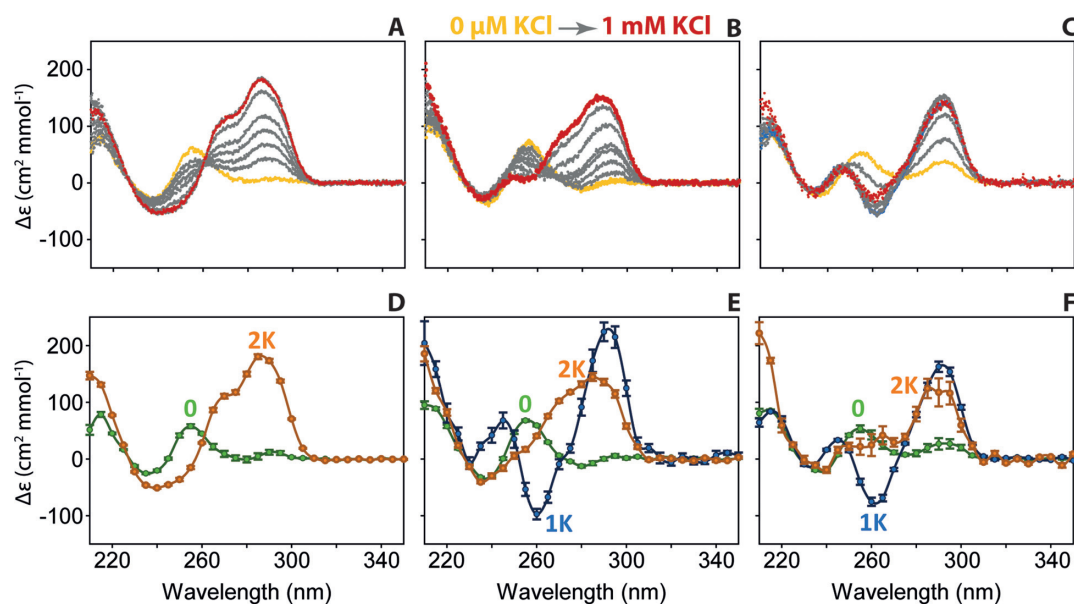
Figure 3. Circular dichroism titrations (20°C) of 10 μM (A) 24TTG, (B) 23TAG and (C) 22GT in 100 mM TMAA with increasing amount of KCl (0 in yellow, 25, 50, 75, 100, 200, 500 and 1000 μM KCl in red). (D–F), CD spectra reconstructed for the 0-K + (green), 1-K + (blue) and 2-K + (orange) complexes, for sequences (D) 24TTG (the 1-K + complex was not abundant enough to reconstruct a CD spectrum), (E) 23TAG and (F) 22GT.
