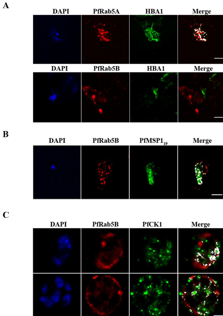
Figure 5. PfRab5B colocalises with PfMSP1 and PfCK1, but not with haemoglobin. (A) PfRab5A colocalises with haemoglobin (HBA1) containing vesicles ( r=0.724 ), unlike PfRab5B ( r=0.081 ; n=3 ). (B) PfRab5B colocalises to differing degrees ( r=0.849 ; n=3 ) with the C-terminal 19 kDa fragment of PfMSP1 on structures close to the food vacuole and the parasite nucleus shown in blue by DAPI staining. (C) PfRab5B colocalises with PfCK1 on intracellular structures ( r=0.615 ; n=3 ) and at the parasite plasma membrane ( r=0.475 ; n=3 ). Areas of colocalisation are shown in white and used to calculate Pearson's r coefficients. Scale bars, 2 \mu m. doi:10.1371/journal.pone.0087695.g005
