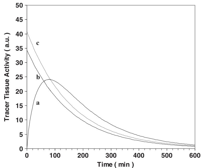
Figure 1 Model comparison. Curve (a) Trapped tracer activity (in arbitrary unit) versus time (in minutes) from Equation 3, assuming irreversible trapping, and the input function of Vriens et al. for ^{18}\text{F} -FDG was used [15]. Curve (b) (full line) Z-F function, i.e. A_{\text{Tot}}(t = 60) * \exp(-\lambda t) (the value for A_{\text{Tot}}(t=60) was taken from curve a). Curve (c) (dotted line) Z-F function with A_{\text{Tot}}(t = 84) (instead of A_{\text{Tot}}(t = 60) ) that gives similar AUC for the two models.
