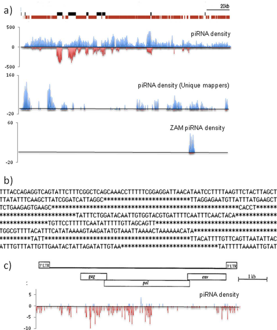
Figure 2 NucBase identified piRNAs mapping to the flamenco locus. (a) Density of annotated transposons of the flamenco locus (X:21501186..1684449) (revised from Brenneke et al. , 2007) indicating sense (Black) and antisense (red) transposon fragments. Density of all piRNAs, the unique mappers piRNAs and ZAM piRNAs (blue: sense - red: antisense) along the flamenco locus from the 2008 Brenneke piRNA database. (b) A representative view of a flamenco fragment (X:21503826..21504465). Asterisks indicate the location of read matches with the reference flamenco sequence. The unmatched sequences are immediately visualized. (c) Organization of the ZAM element with locations of the different ORFs and piRNAs density along the ZAM sequence.
