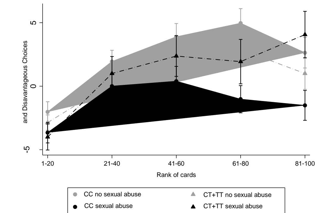
Figure 2: Interaction between rs1396862 within CRHR1 and childhood sexual abuse on IGT scores.
